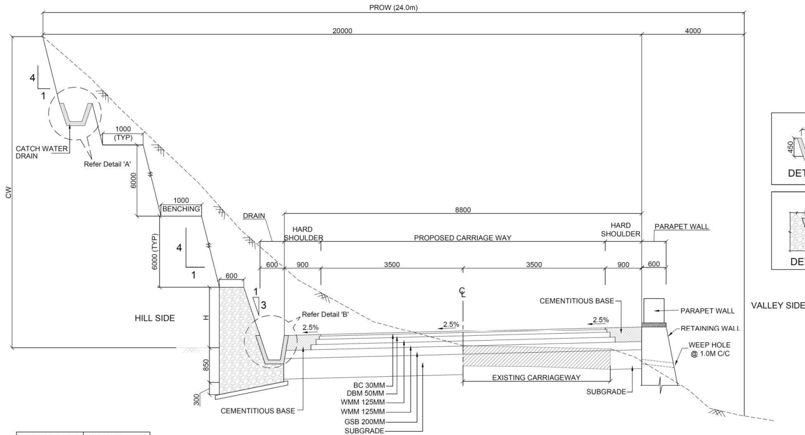
TCS - 2 TYPICAL CROSS SECTION RECONSTRUCTION / WIDENING OF 2 LANE WITH HARD SHOULDER IN RURAL AREA (WITH BREST WALL ON HILL SIDE AND RETAINING WALL ON VALLEY SIDE )
